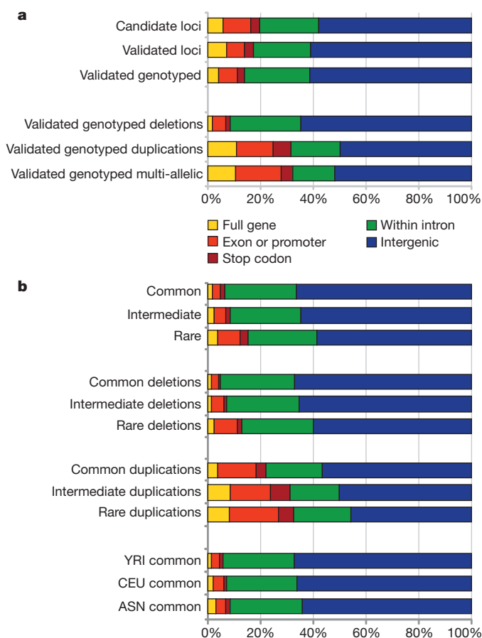
Figure 2 | Functional impact of CNVs by type, frequency and population.
